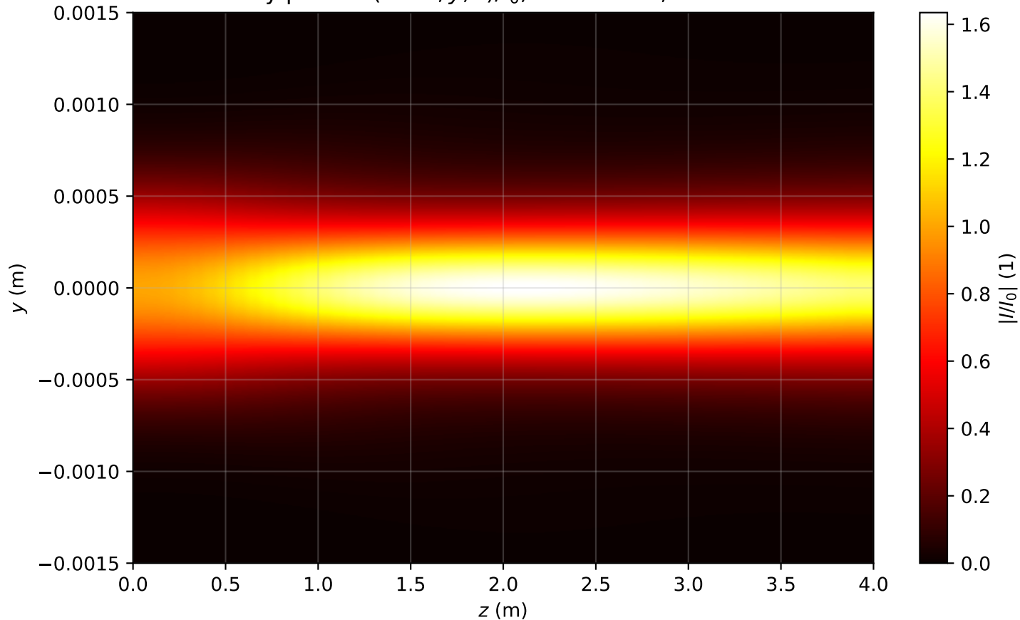
Intensity profile I(x=0, y, z)/I_0 , P_{in}=0.9P_{cr} , artificial time
